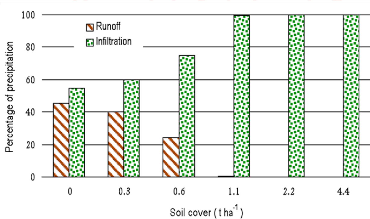
Effect of amount of soil cover on rainwater runoff and infiltration.
